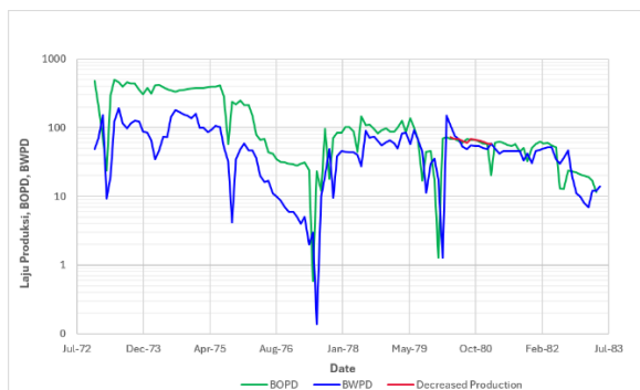
Figure 5. Graph of the results of semilog scale digitization in determining oil reserves.
