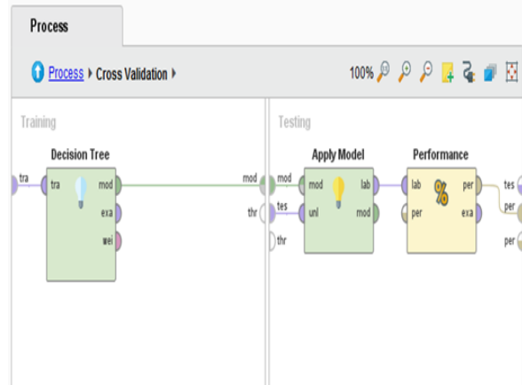
Sumber: (Angraini Yeni, Fauziah Siti, 2020) Gambar2. Model validasi DT
