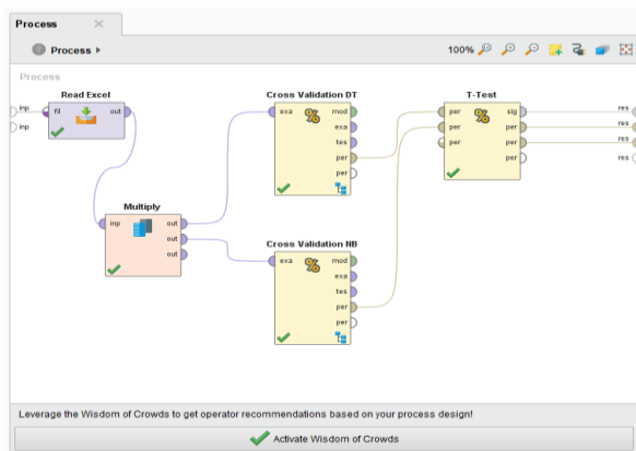
Figure 1. Testing Data Mining with Rapid Miner
