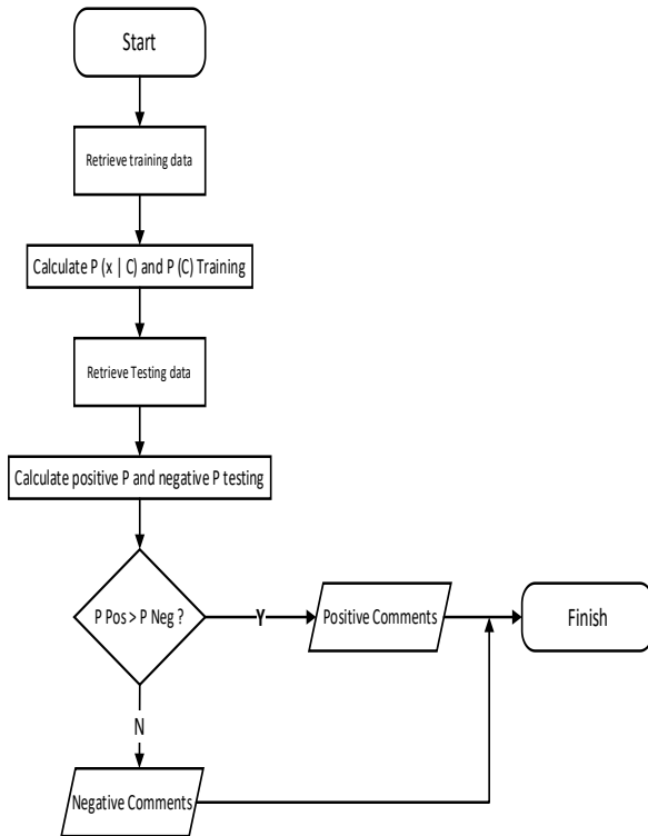
Figure 1. Algorithm workflow of Naive Bayes
