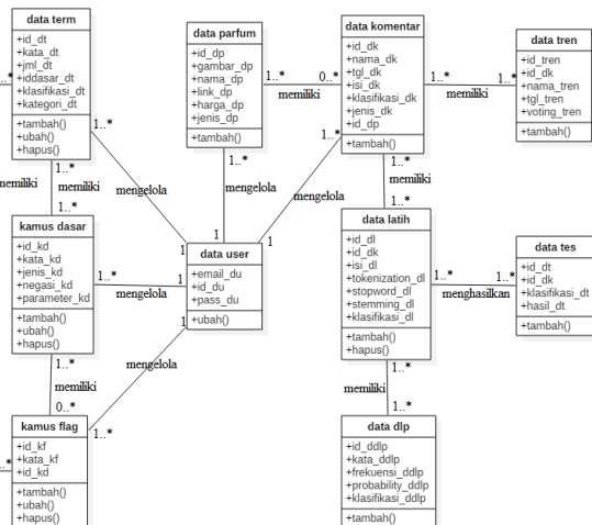
Figure 3. Class diagram of the opinion mining system
