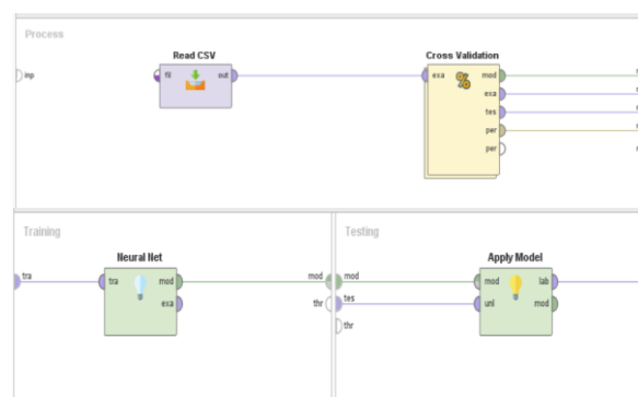
Figure 8. Testing binary classification and 5-level classification approaches with the NN algorithm
