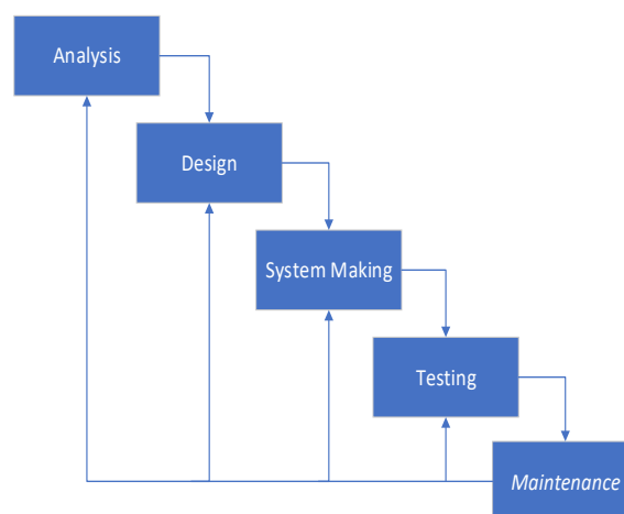
Figure 1. Waterfall Methods
