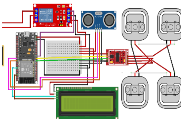
Figure 4. Box Locking System Circuit
