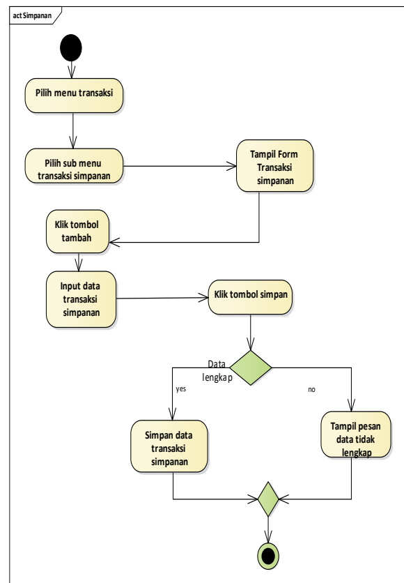
Sumber: (Safitri et al., 2018) Gambar 5. Activity Diagram Sistem Informasi Menu Simpanan
