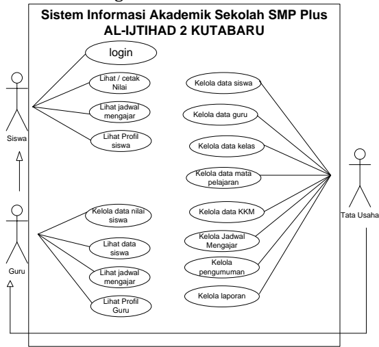
Sumber (Riki, Sari, & Indriani, 2017) Gambar1. Use Case Diagram Sistem Informasi Akademik
