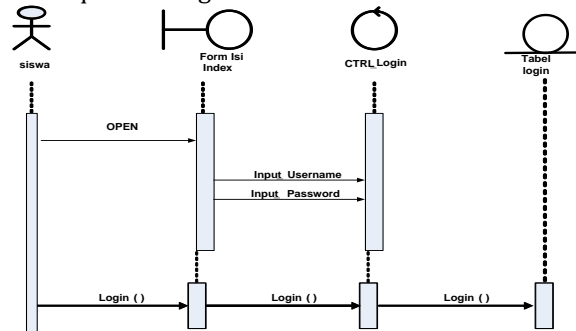
Sumber (Riki, Sari, & Indriani, 2017) Gambar 3. Sequence halaman login
