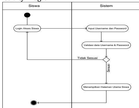
Sumber (Riki, Sari, & Indriani, 2017) Gambar 2. Activity Diagram login siswa
