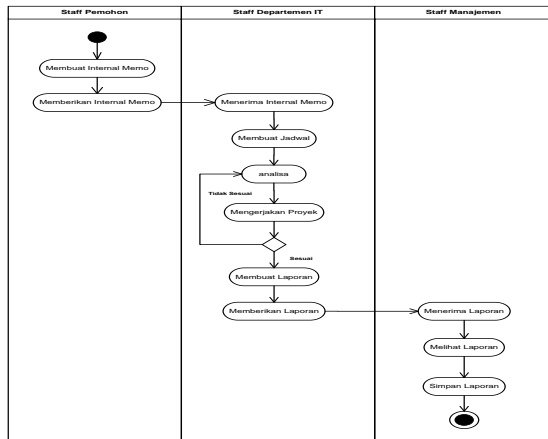
Sumber: (Septiani,2018) Gambar 1. Activity Diagram Sistem Berjalan Departemen IT
