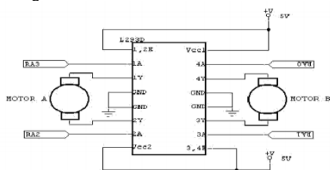
Gambar 6 Rangkaian Driver Motor DC
