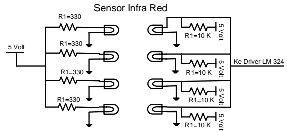
Sumber: Rosano, Yunita & Raharjo (2016) Gambar 2. Sensor Infra Red
