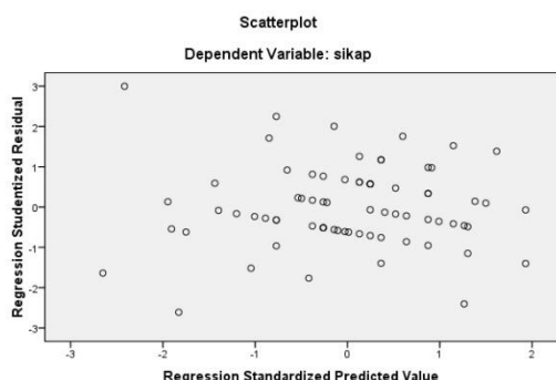
Gambar 2. Output Scatterplot
