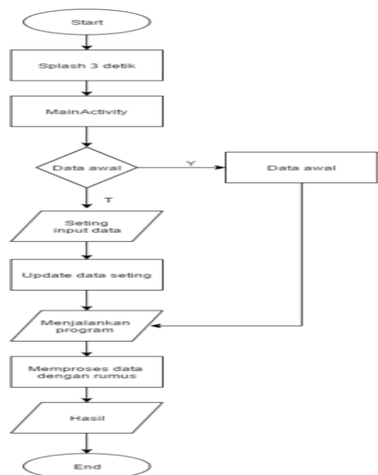
Sumber: hasil analisis(2016) Gambar 3. Activity Diagram
