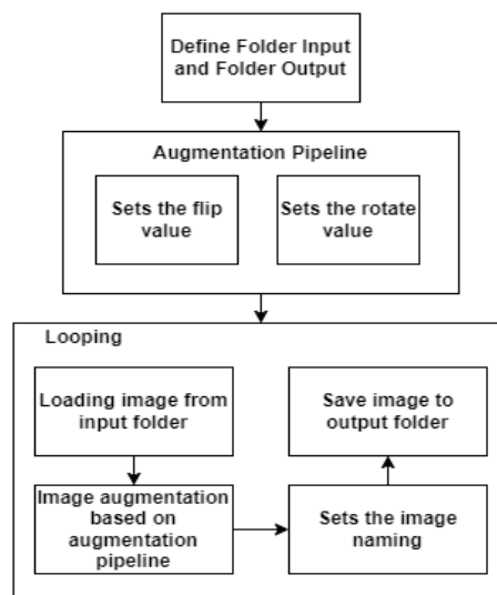
Figure 2. Data Augmentation Flowchart
