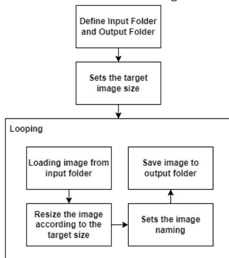
Figure 3. Data Resizing Flowchart
