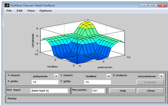
Sumber: (Ma'arif, Samsul ; Sfenrianto; Prayitno, 2019) Gambar 17. Tampilan Surface Viewer
