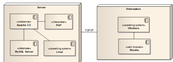
Gambar 5. Deployment Diagram
