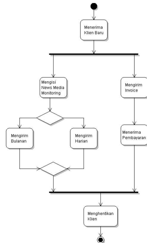
Gambar 4. Activity Diagram Prosedur Pengiriman News Media Monitoring
