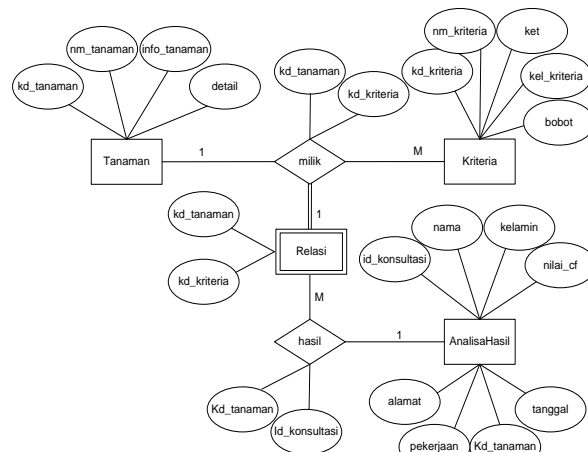
Source: (Ramdhani, Susilawati, & Saputra, 2020) Figure 5. ERD Expert System Application
