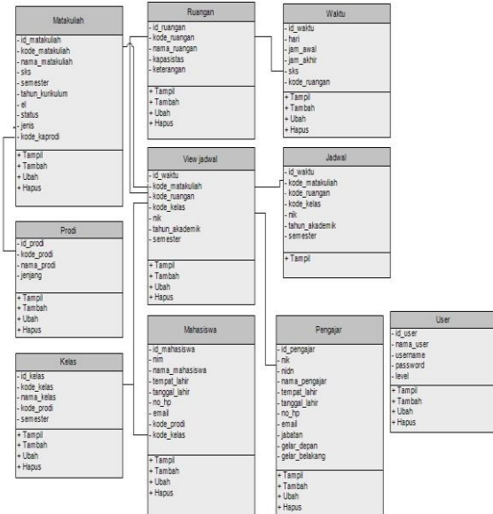
Source: (Zaeniah & Salman, 2020) Figure 3. Class Diagram
