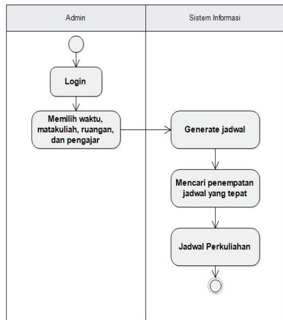
Source: (Zaeniah & Salman, 2020) Figure 4. Activity Diagram
