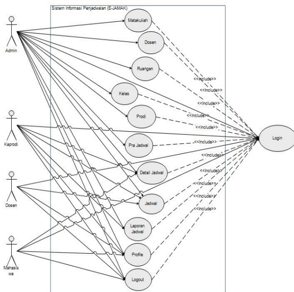
Source: (Zaeniah & Salman, 2020) Figure 2. Use Case Diagram
