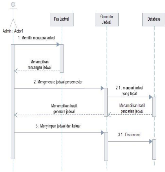
Source: (Zaeniah & Salman, 2020) Figure 5. Sequence Diagram
