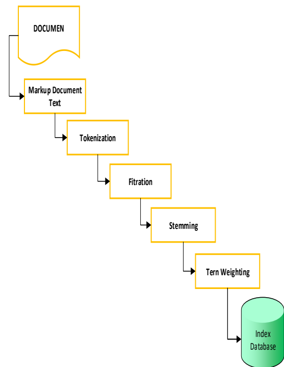
Gambar 5. Proses Tokenization.
