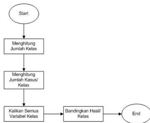
Gambar 1. Flowchart Algoritma Naïve Bayes
