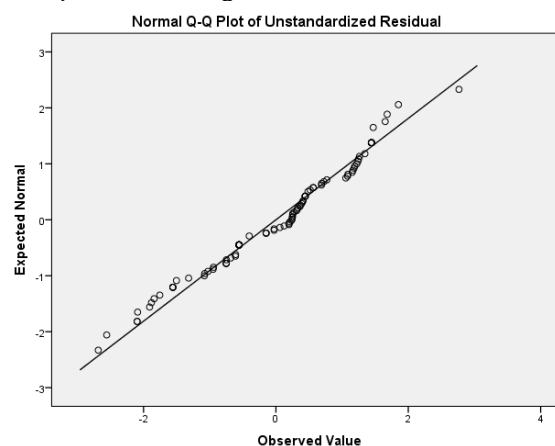
Gambar 1. Grafik normal probability plot
