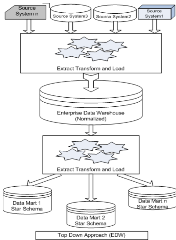
(Sumber : http://www.DWHInfo.com ) Gambar 2. Pendekatan Top-Down .
