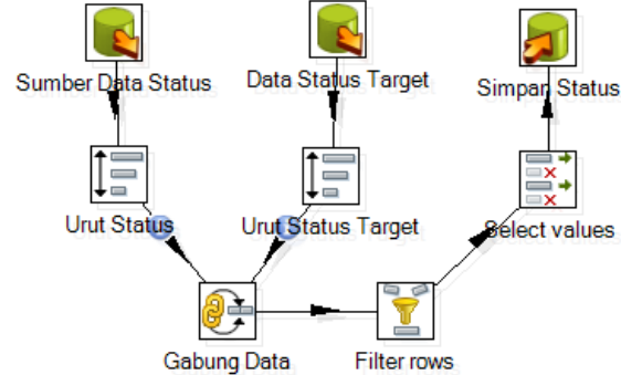
Sumber : Hasil Penelitian (2015) Gambar 13. Staging data dimensi status.
