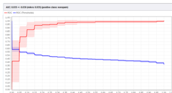
Gambar 11. Kurva ROC dengan Support Vector Machine dan Support Vector Machine berbasis Particle Swarm Optimization
