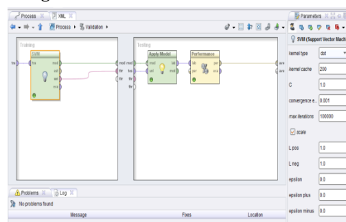
Gambar 7. Model Pengujian validasi Support Vector Machine
