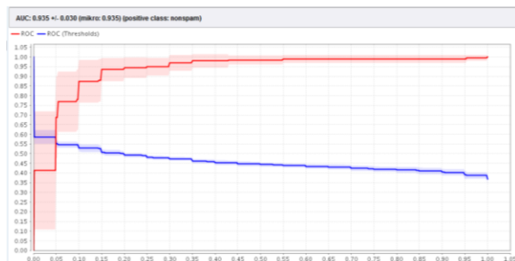
Gambar 10. Kurva ROC dengan Metode Support Vector Machine berbasis Particle Swarm Optimization (PSO)
