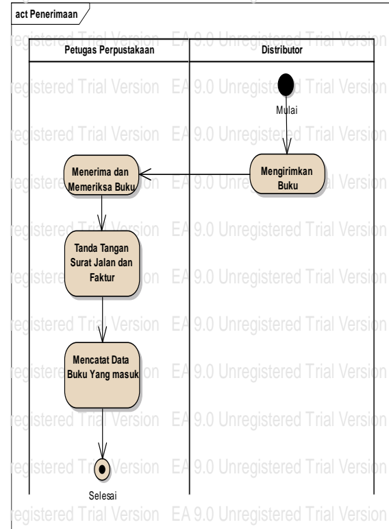
Gambar 5. Activity Diagram Penerimaan Buku.
