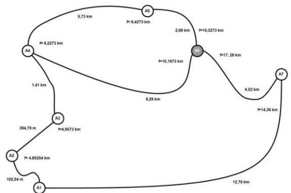
Figure 4. A-Star Algorithm Graph (Final)
