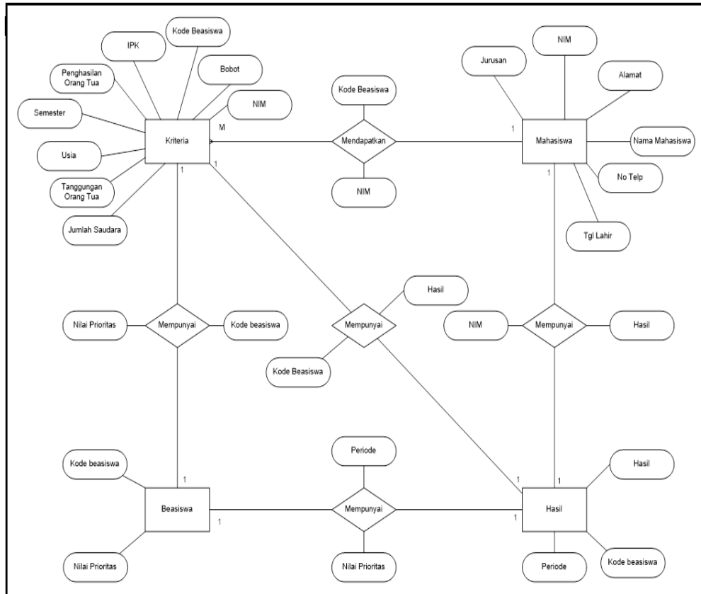
Gambar.3.EntityRelationship Diagram (ERD)
