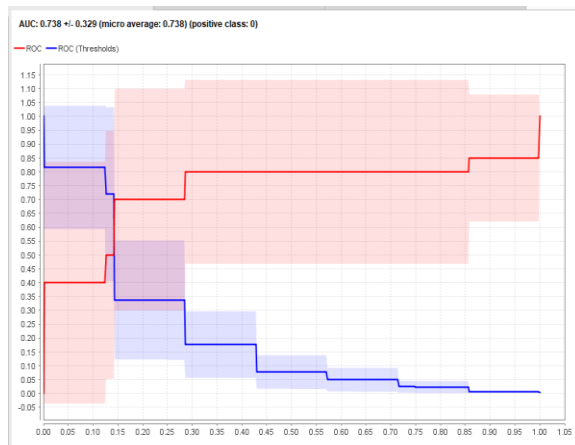
Figure 10. AUC eural Network Curve
