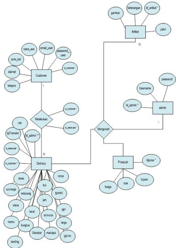
Gambar 13. ERD Pelayanan Cargo
