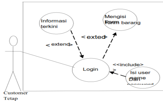
Sumber: (Hasil Penelitian, 2015) Gambar 7. Use Case Diagram Pengiriman barang customer tetap
