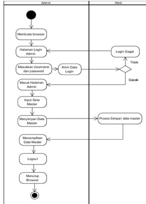
Sumber : Fitriani (2018) Gambar 5. Activity Diagram Penginputan Data Master
