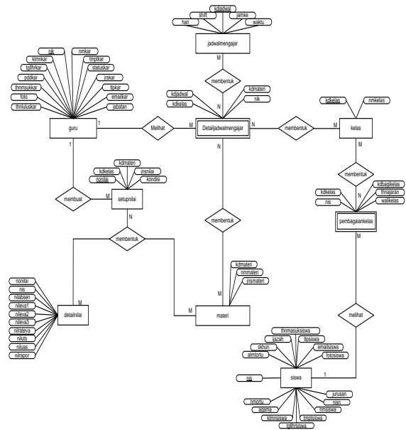
Sumber : Fitriani (2018) Gambar 9. Entity Relationship Diagram
