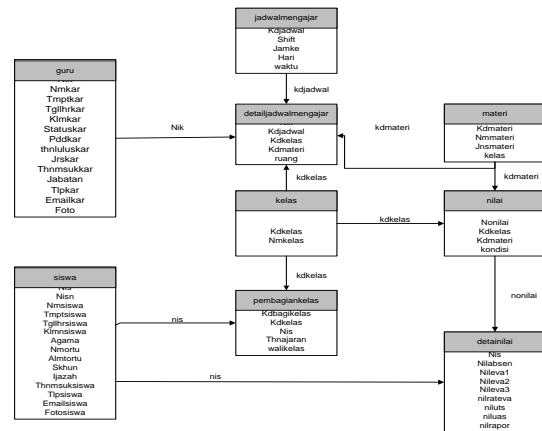
Sumber : Fitriani (2018) Gambar 10. Logical Record Structure
