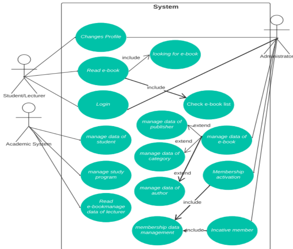
Gambar 6. Usecase Diagram
