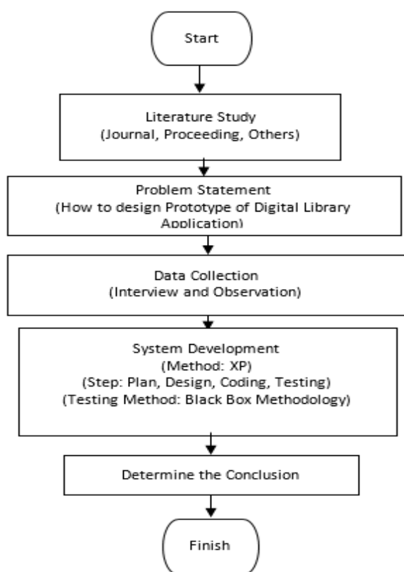
Figure 2. Research Framework
