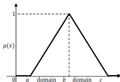
Figure 3. Graph of Triangle Linear Functions
