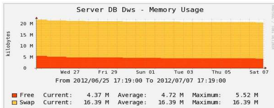
Gambar 6. Memory Usageselbelum mekanisme Load-balancing Clusters
